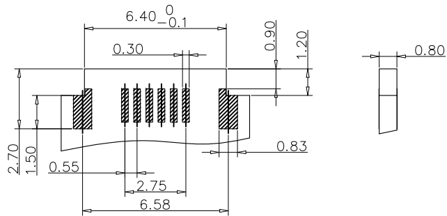
RECOMMENDED PCB LAYOUT(COMPONENT SIDE) TOLERANCE FOR PCB LAYOUT IS \pm 0.05
