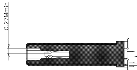
SECTION-A-A SCALE 1:1
