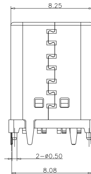
SECTION-A-A SCALE 1:1
